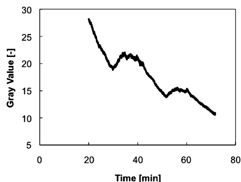
Figure 5. Oscillating profile of fluorescence intensity for self-oscillating polymer brush modified slide glass. The polymer brush surface contacts the solution containing MA (0.1 M), \text{NaBrO}_3 (0.15 M) and \text{HNO}_3 (0.81 M) at 18 °C.
